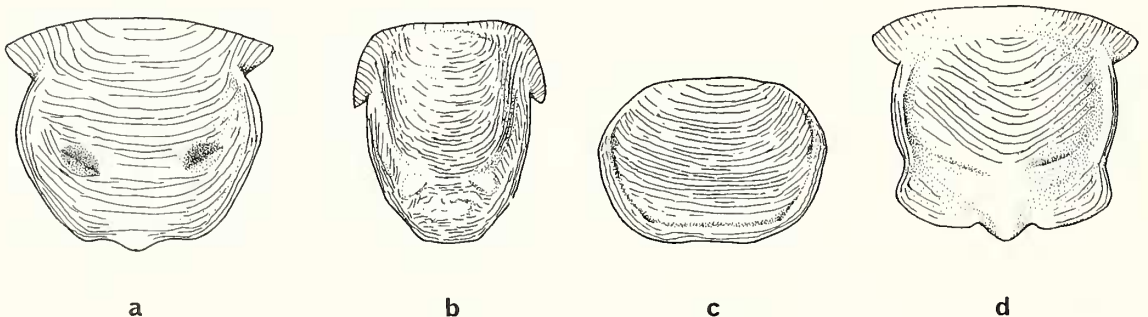
TEXT-FIG. 8. Hypostomes of higher Asaphina illustrating characters 22 and 23 (see Table 2); all these types have well-developed sculpture of terrace ridges on the middle body. a , generalized Nileid hypostome; early Ordovician Porouileus (after Fortey 1975, pl. 13, fig. 8). b , presumed primitive hypostomal morphology of Asaphidae; Upper Cambrian Niobella (after Westergård 1939, pl. 2, fig. 2). c , loss of maculae in Cyclopygidae; early Ordovician Microparia (after Fortey and Owens 1987, fig. 45 b ). d , Taihungshaniidae, showing similarity with Nileidae; early Ordovician Taihungshania (after Courtessole et al. 1981, pl. 4, fig. 7). Two to three times natural size.
